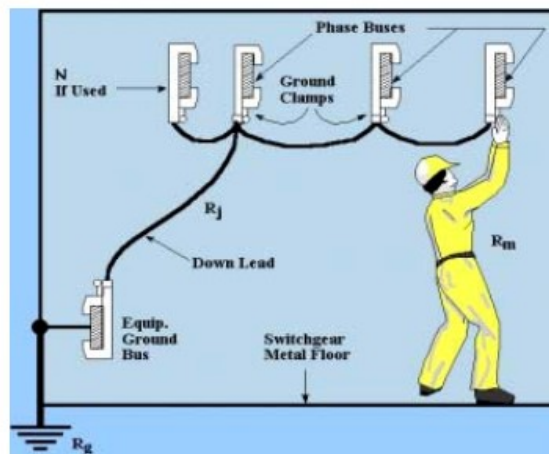
Figure 2 - Grounding Metal Clad Gear
